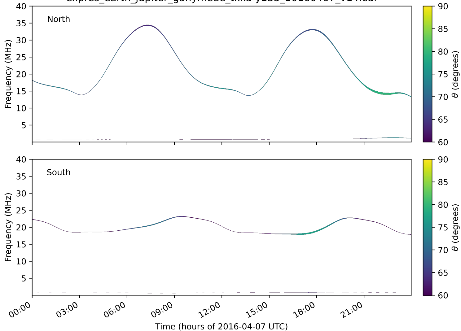
expres_earth_jupiter_ganymede_txka-y235_20160407_v14.cdf
