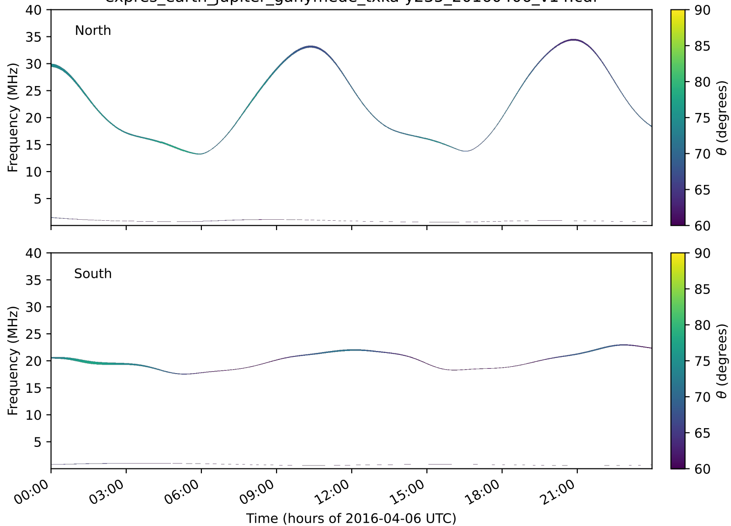
expres_earth_jupiter_ganymede_txka-y235_20160406_v14.cdf
