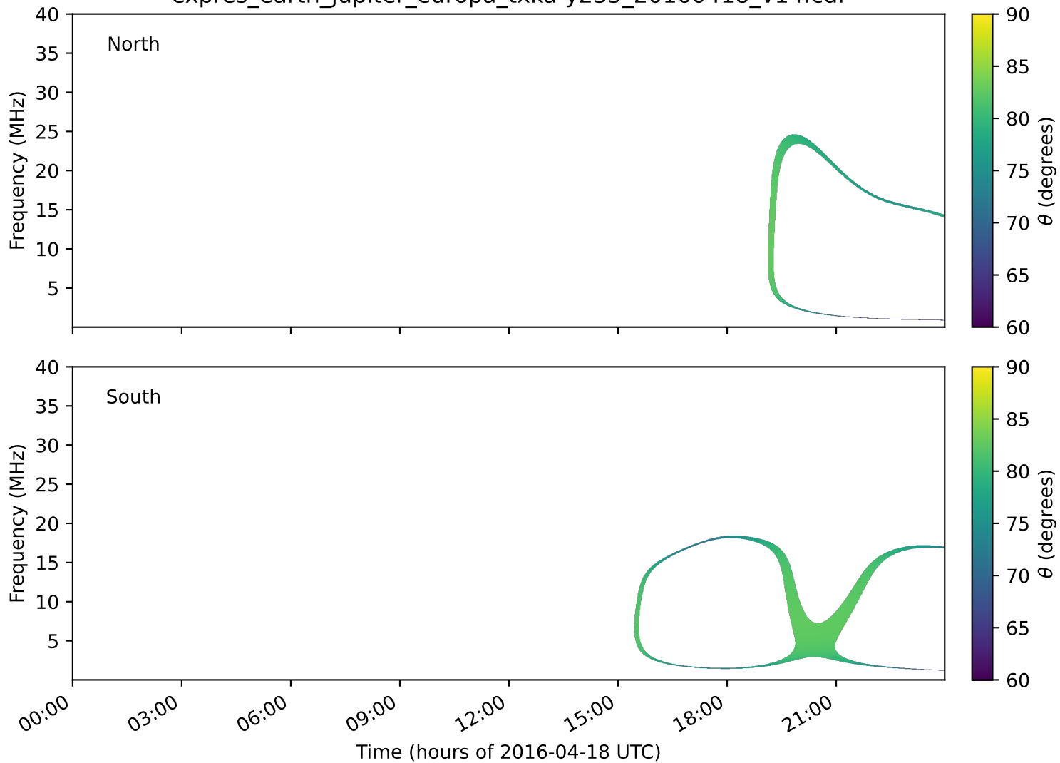
expres_earth_jupiter_europa_txka-y235_20160418_v14.cdf
