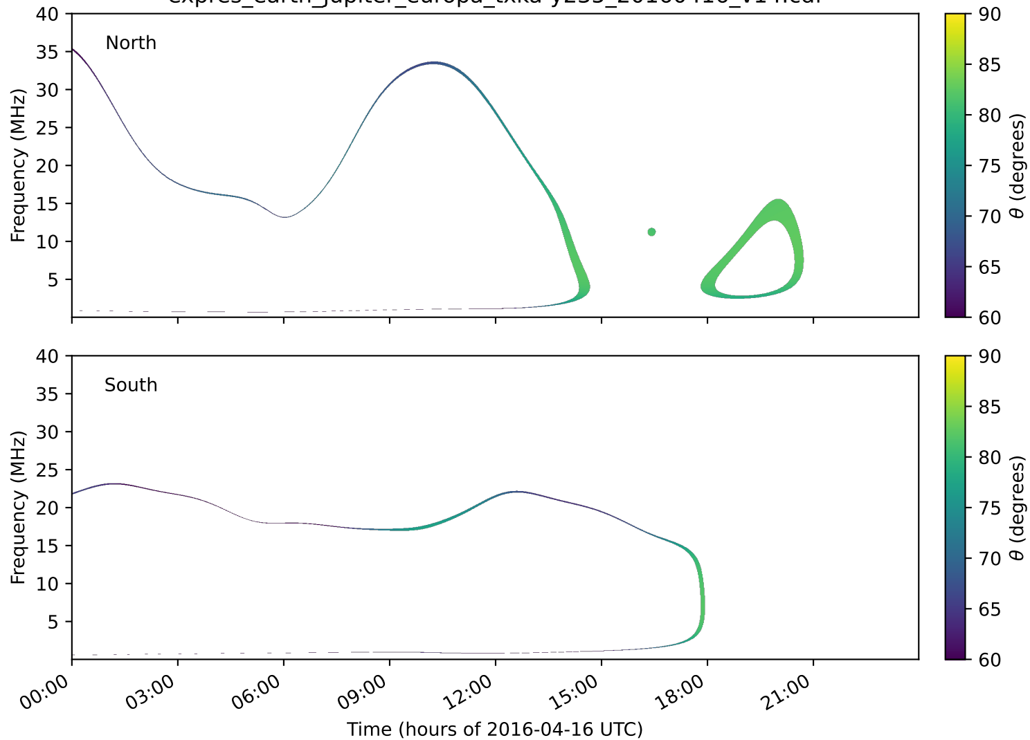
expres_earth_jupiter_europa_txka-y235_20160416_v14.cdf
