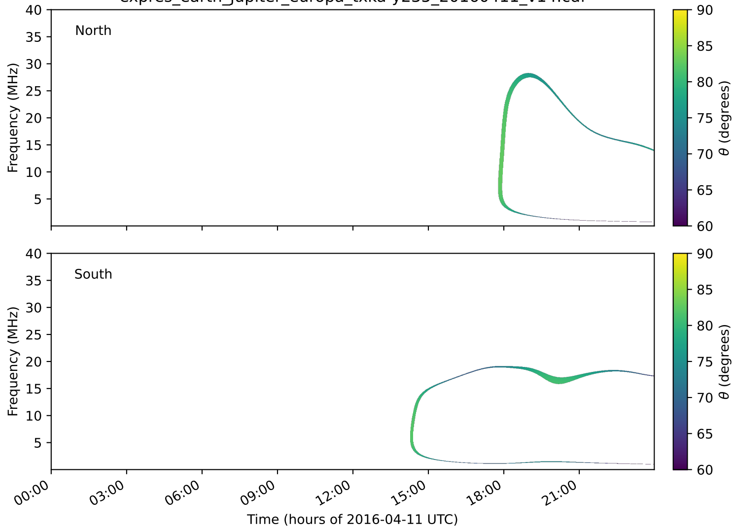
expres_earth_jupiter_europa_txka-y235_20160411_v14.cdf
