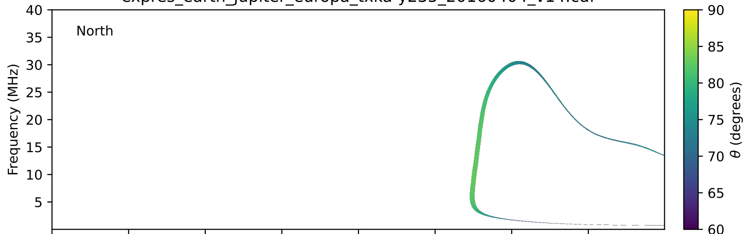
expres_earth_jupiter_europa_txka-y235_20160404_v14.cdf
