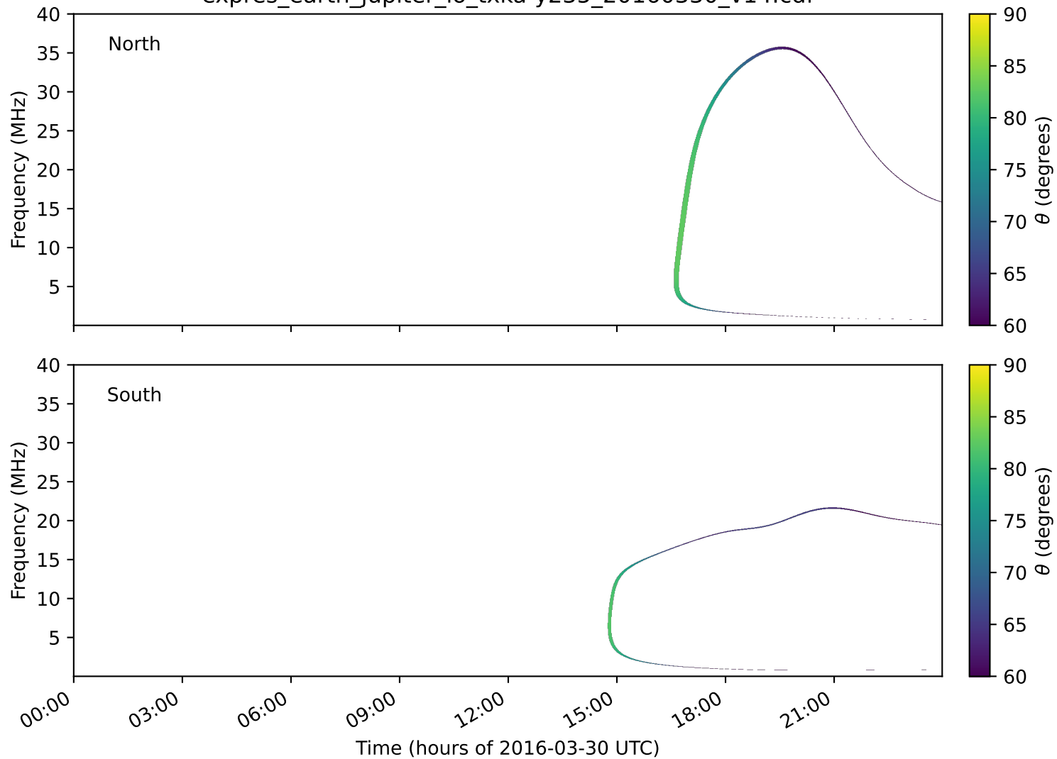
expres_earth_jupiter_io_txka-y235_20160330_v14.cdf
