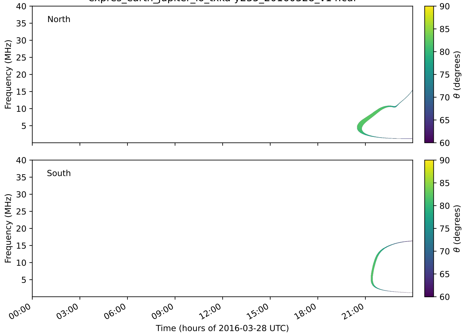
expres_earth_jupiter_io_txka-y235_20160328_v14.cdf
