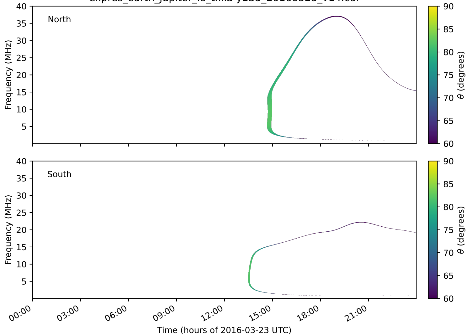
expres_earth_jupiter_io_txka-y235_20160323_v14.cdf
