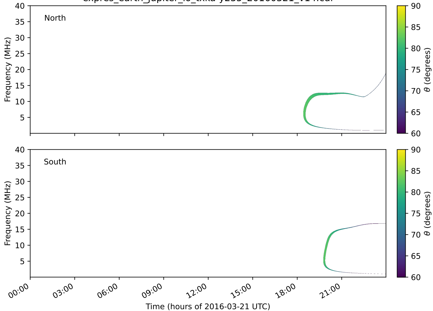
expres_earth_jupiter_io_txka-y235_20160321_v14.cdf
