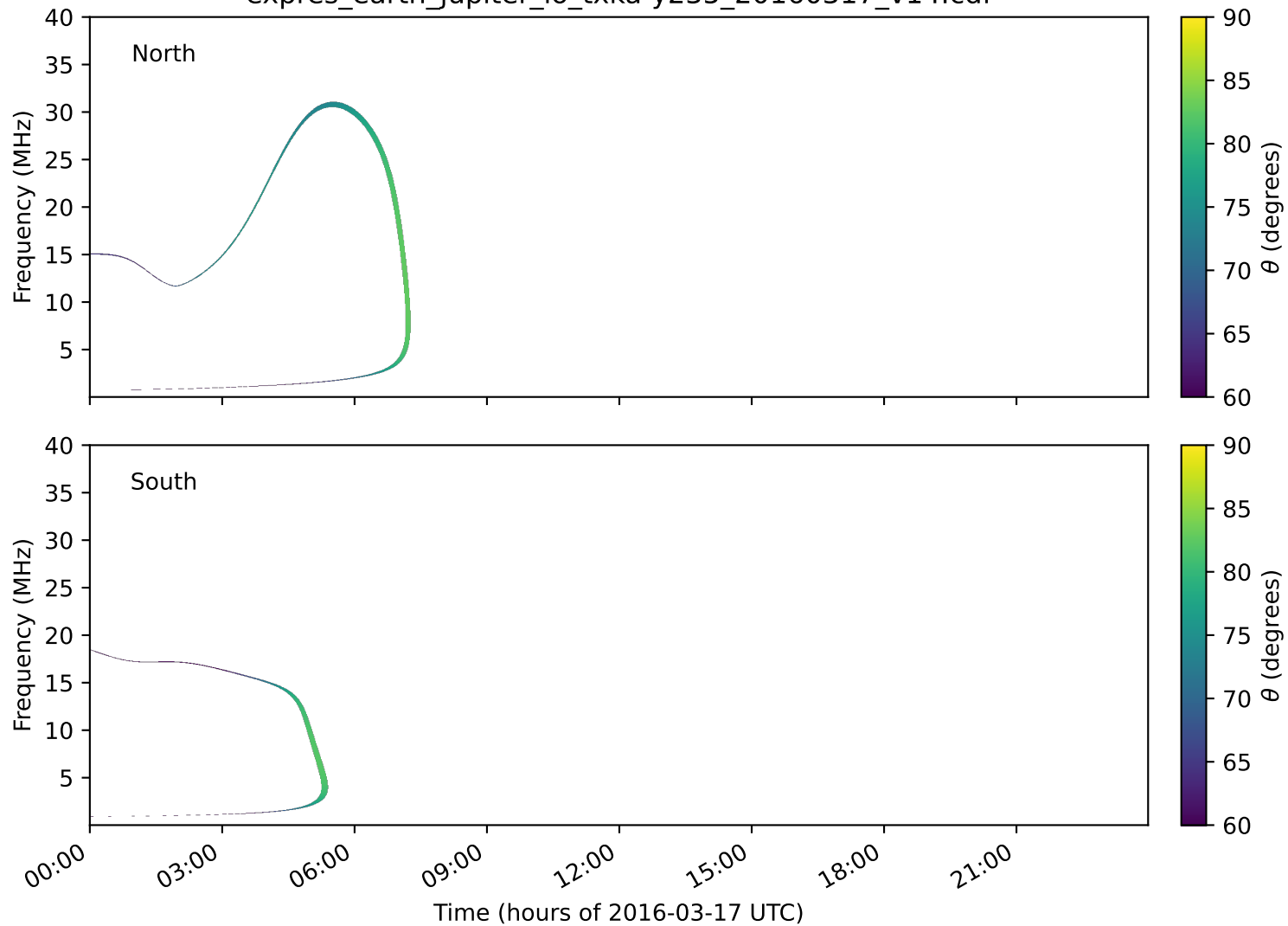
expres_earth_jupiter_io_txka-y235_20160317_v14.cdf
