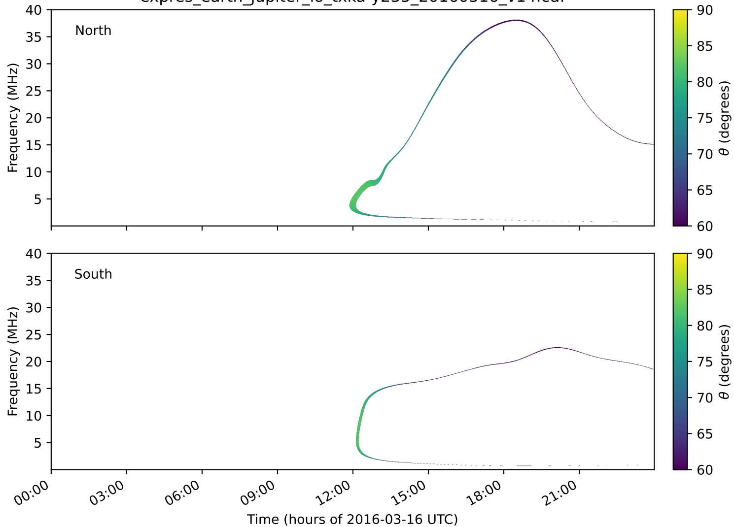
expres_earth_jupiter_io_txka-y235_20160316_v14.cdf
