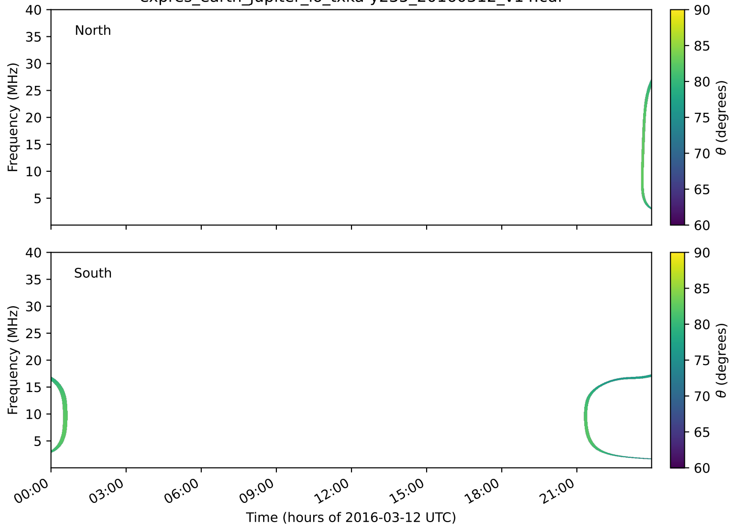
expres_earth_jupiter_io_txka-y235_20160312_v14.cdf
