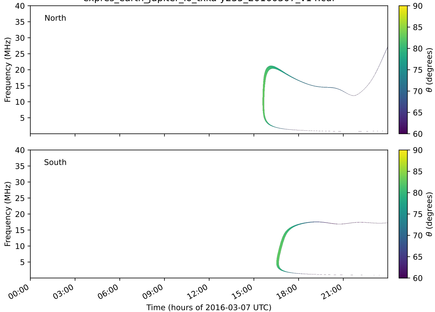
expres_earth_jupiter_io_txka-y235_20160307_v14.cdf
