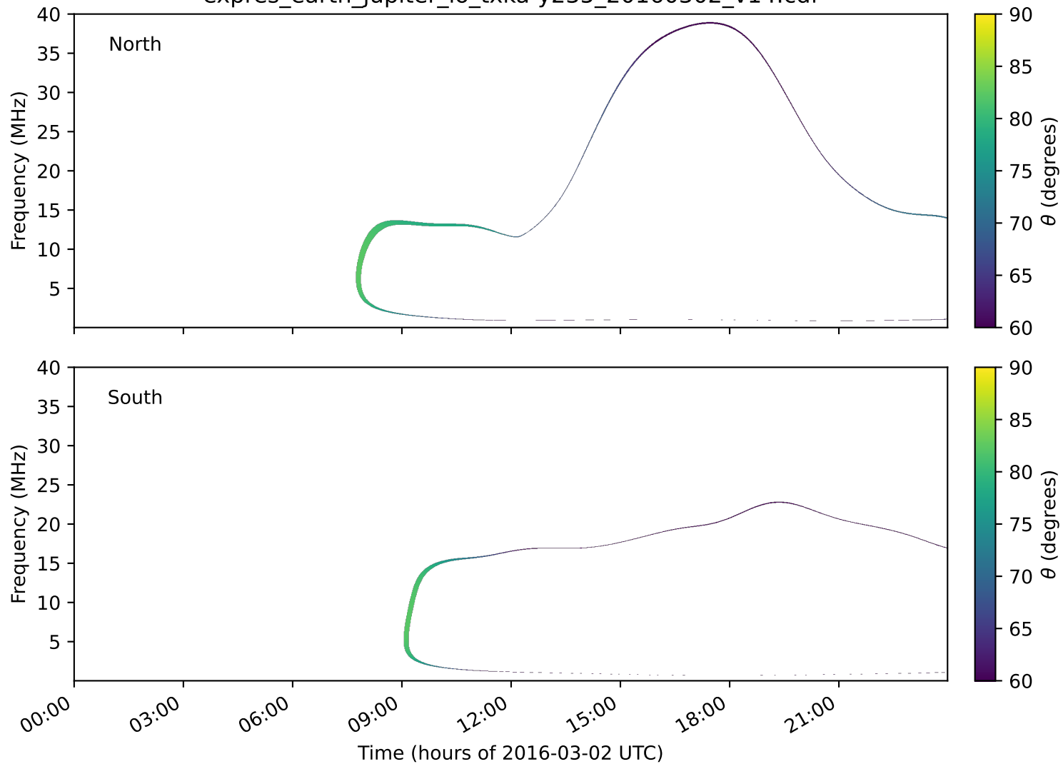
expres_earth_jupiter_io_txka-y235_20160302_v14.cdf
