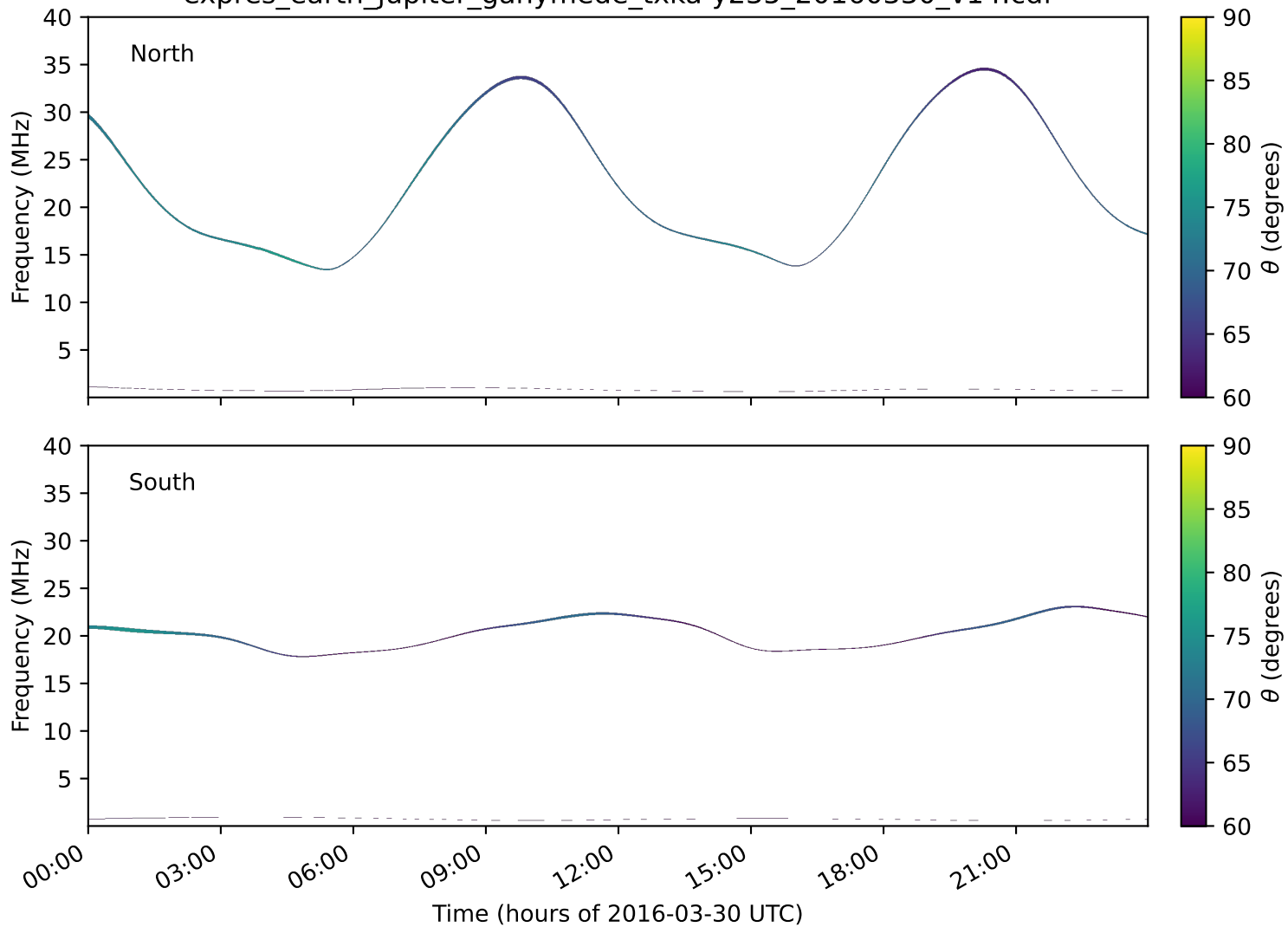
expres_earth_jupiter_ganymede_txka-y235_20160330_v14.cdf
