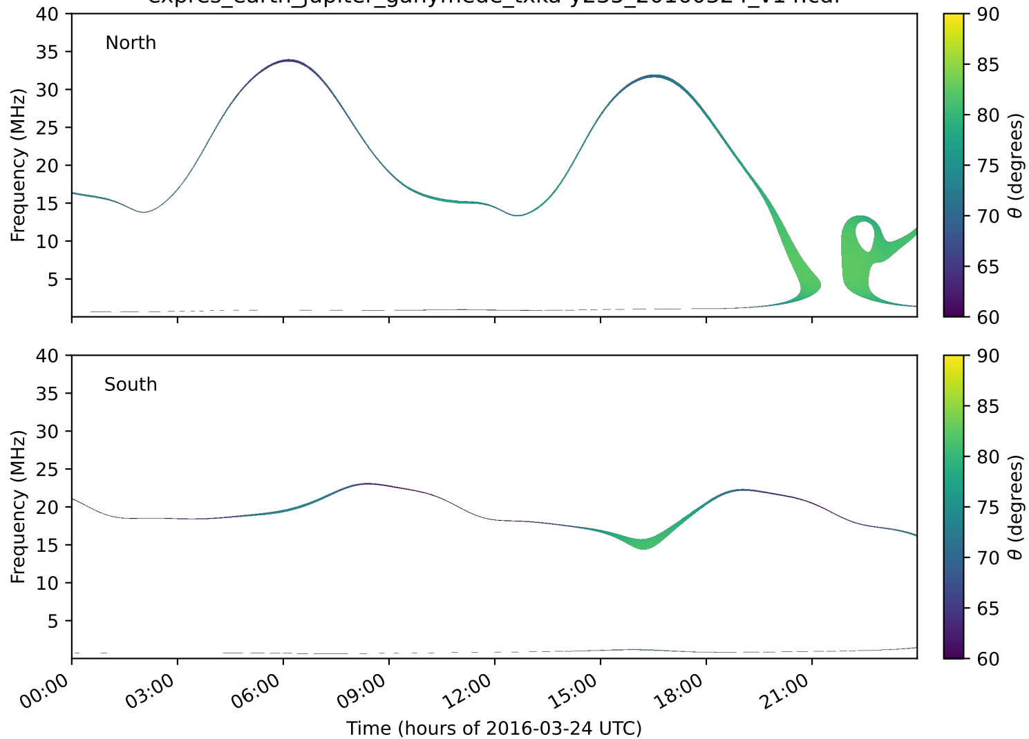
expres_earth_jupiter_ganymede_txka-y235_20160324_v14.cdf
