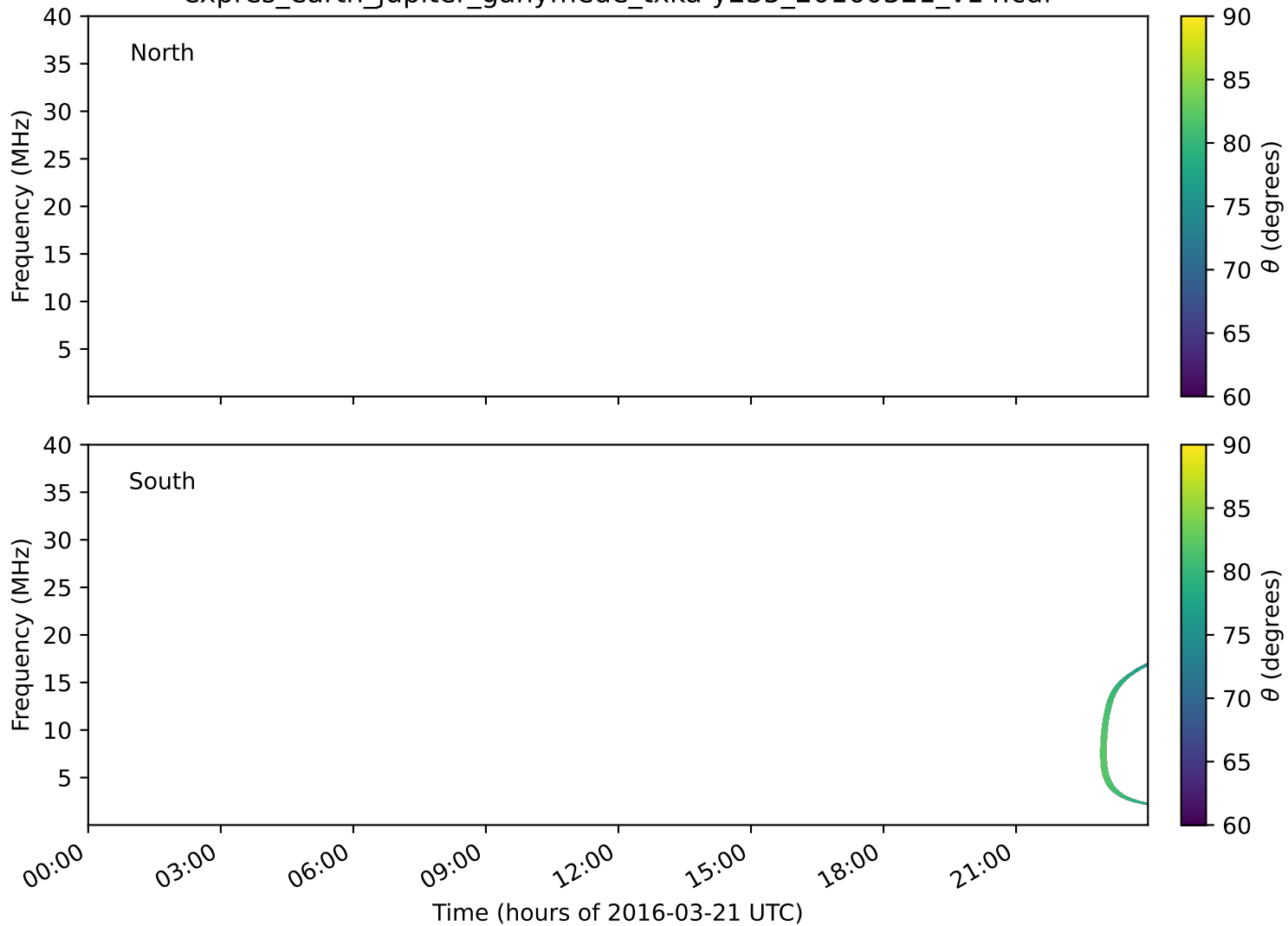
expres_earth_jupiter_ganymede_txka-y235_20160321_v14.cdf
