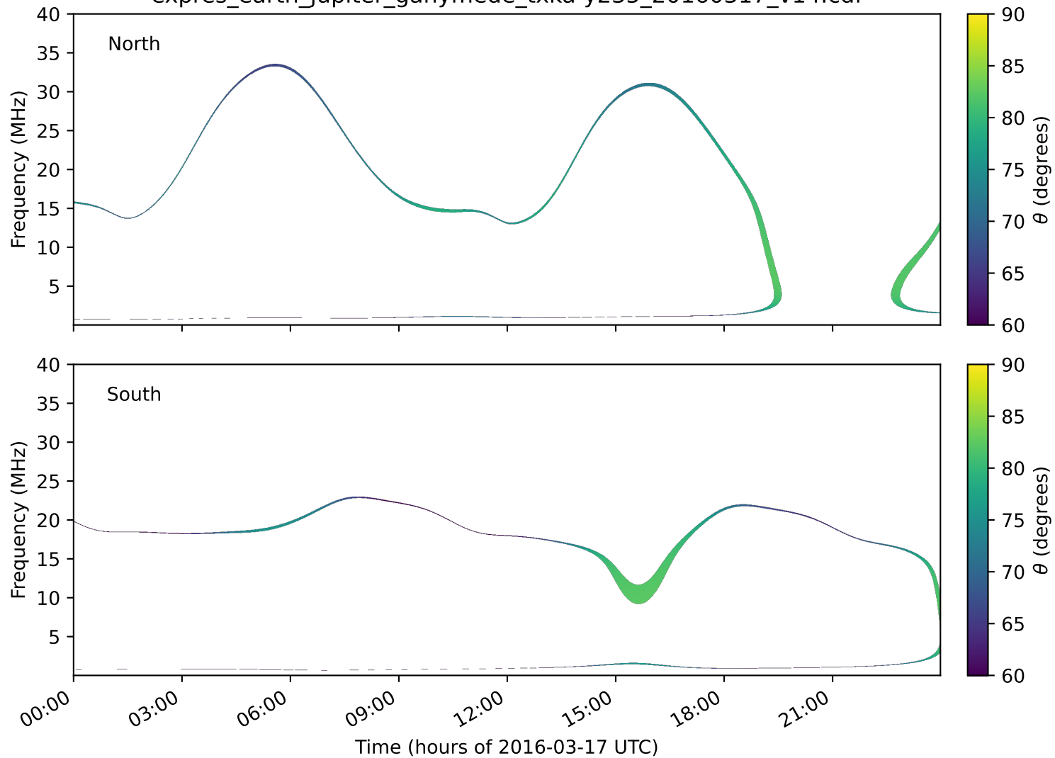
expres_earth_jupiter_ganymede_txka-y235_20160317_v14.cdf
