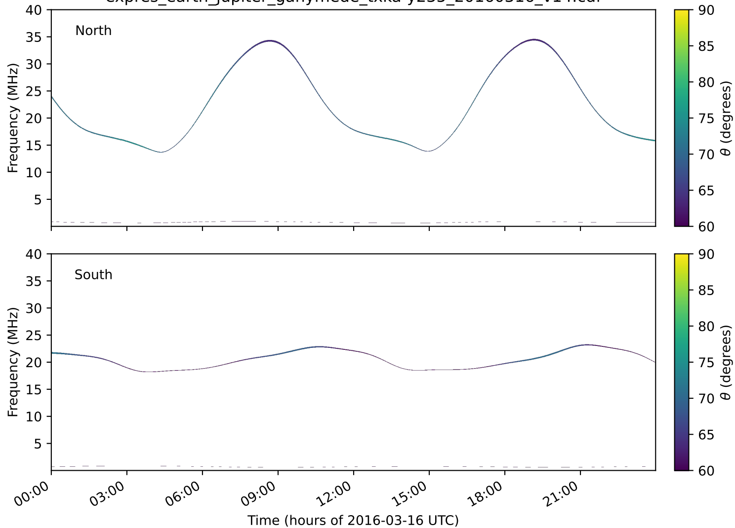
expres_earth_jupiter_ganymede_txka-y235_20160316_v14.cdf
