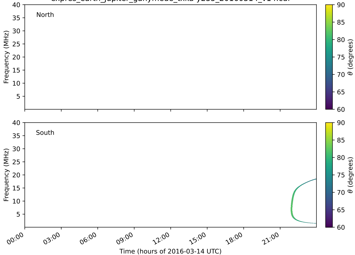
expres_earth_jupiter_ganymede_txka-y235_20160314_v14.cdf
