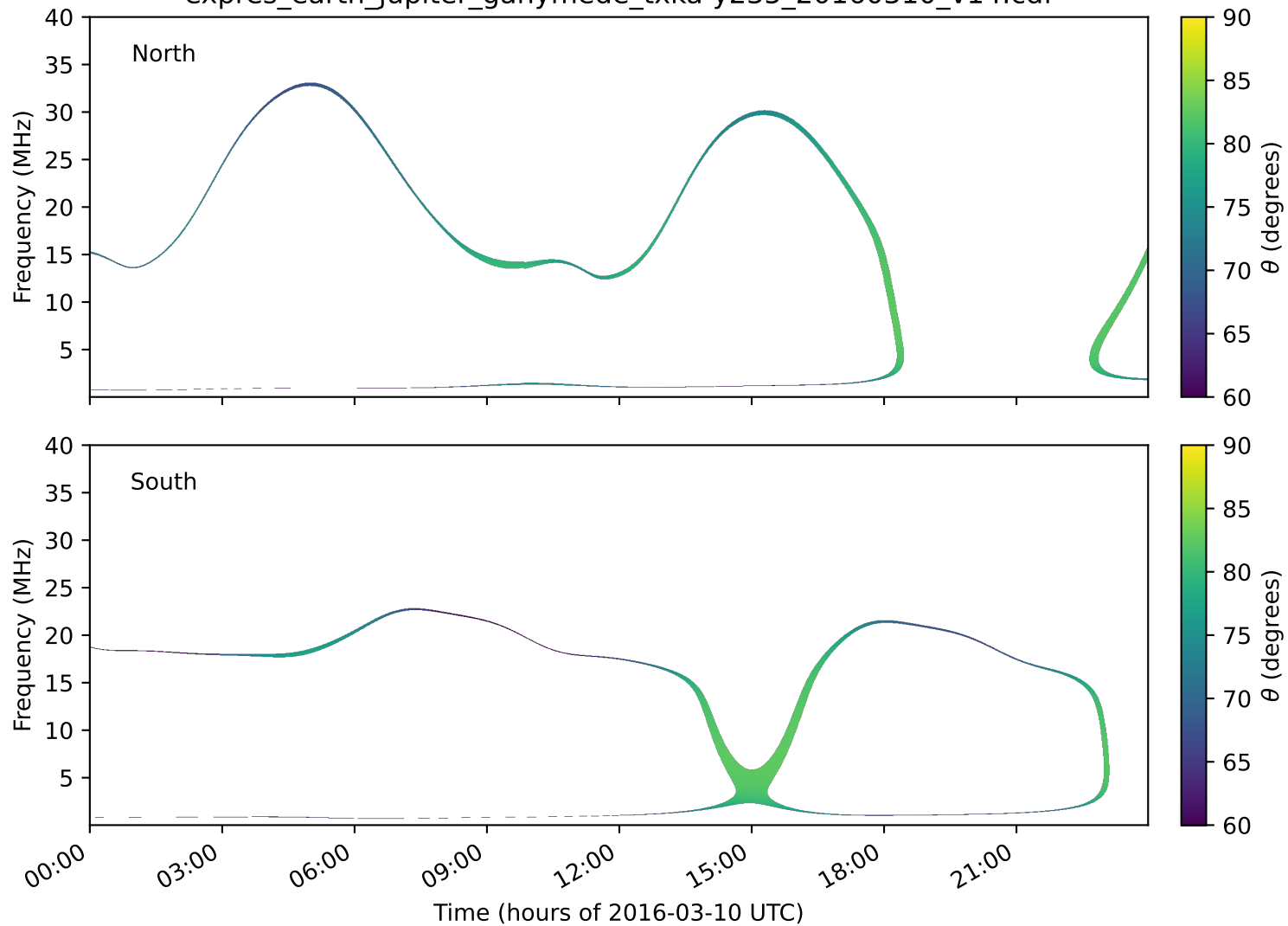
expres_earth_jupiter_ganymede_txka-y235_20160310_v14.cdf
