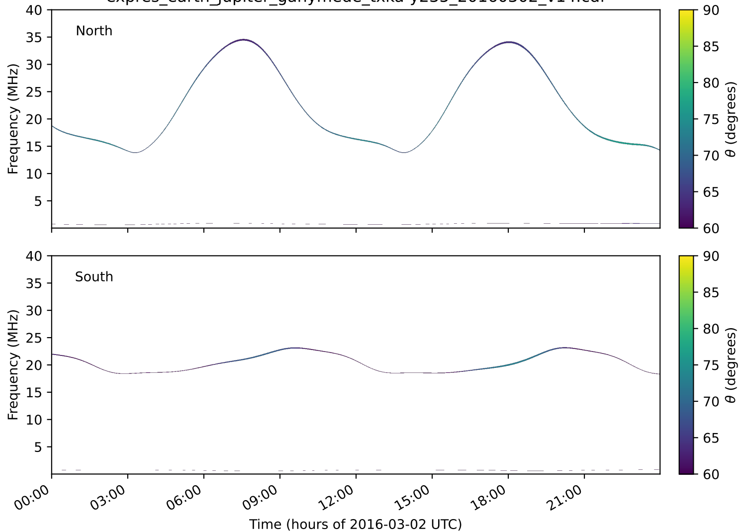
expres_earth_jupiter_ganymede_txka-y235_20160302_v14.cdf
