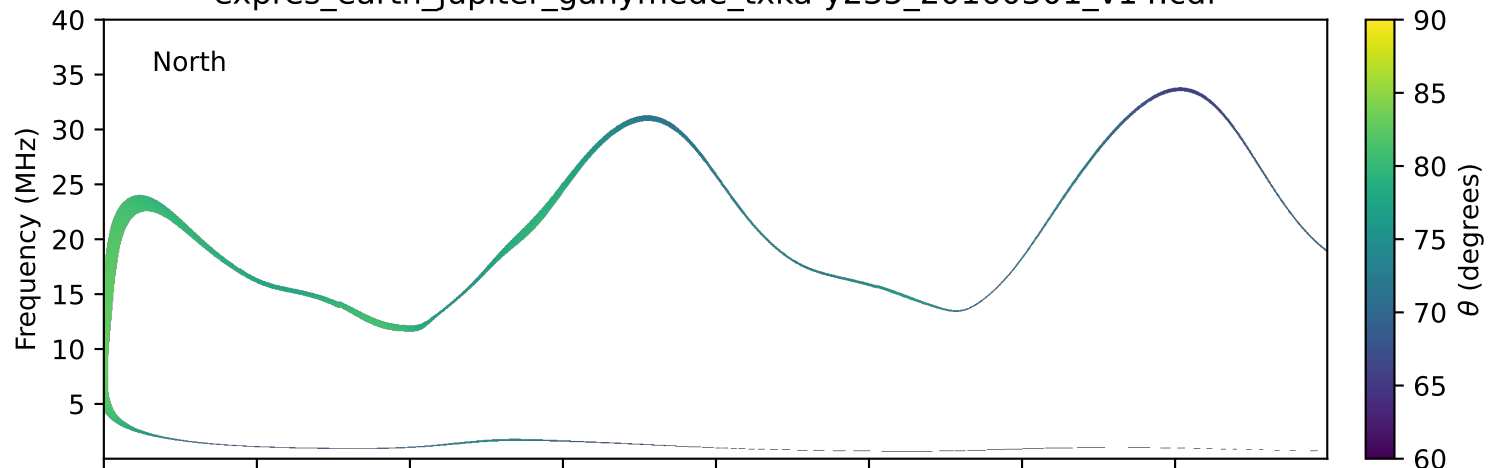
expres_earth_jupiter_ganymede_txka-y235_20160301_v14.cdf
