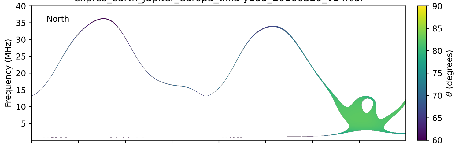
expres_earth_jupiter_europa_txka-y235_20160329_v14.cdf
