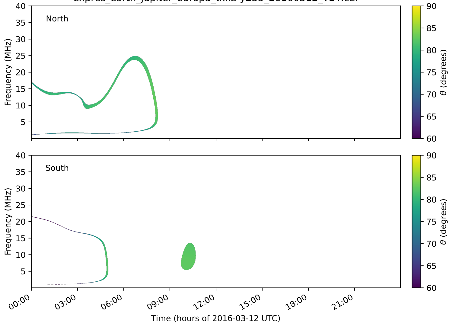
expres_earth_jupiter_europa_txka-y235_20160312_v14.cdf
