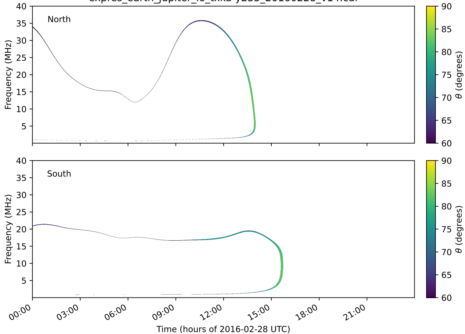
expres_earth_jupiter_io_txka-y235_20160228_v14.cdf
