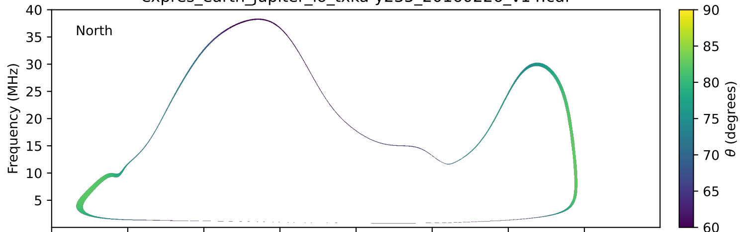
expres_earth_jupiter_io_txka-y235_20160226_v14.cdf
