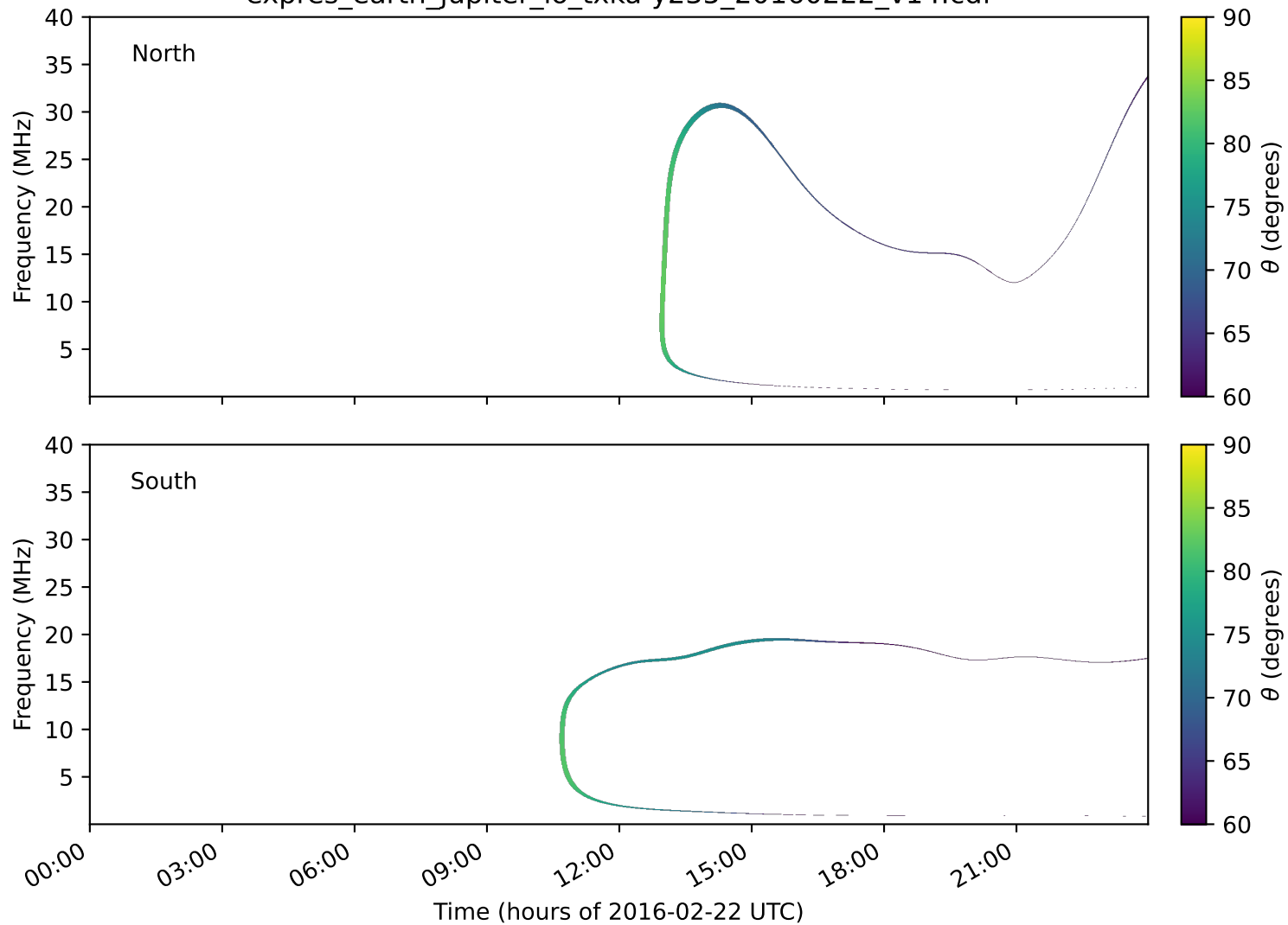
expres_earth_jupiter_io_txka-y235_20160222_v14.cdf
