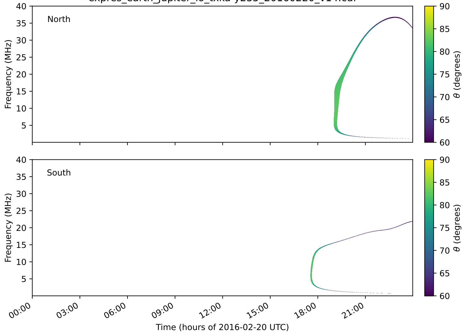
expres_earth_jupiter_io_txka-y235_20160220_v14.cdf
