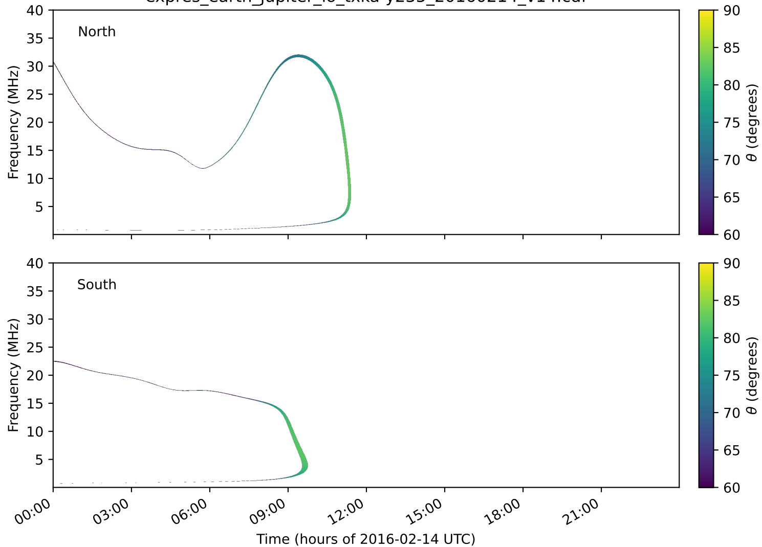
expres_earth_jupiter_io_txka-y235_20160214_v14.cdf
