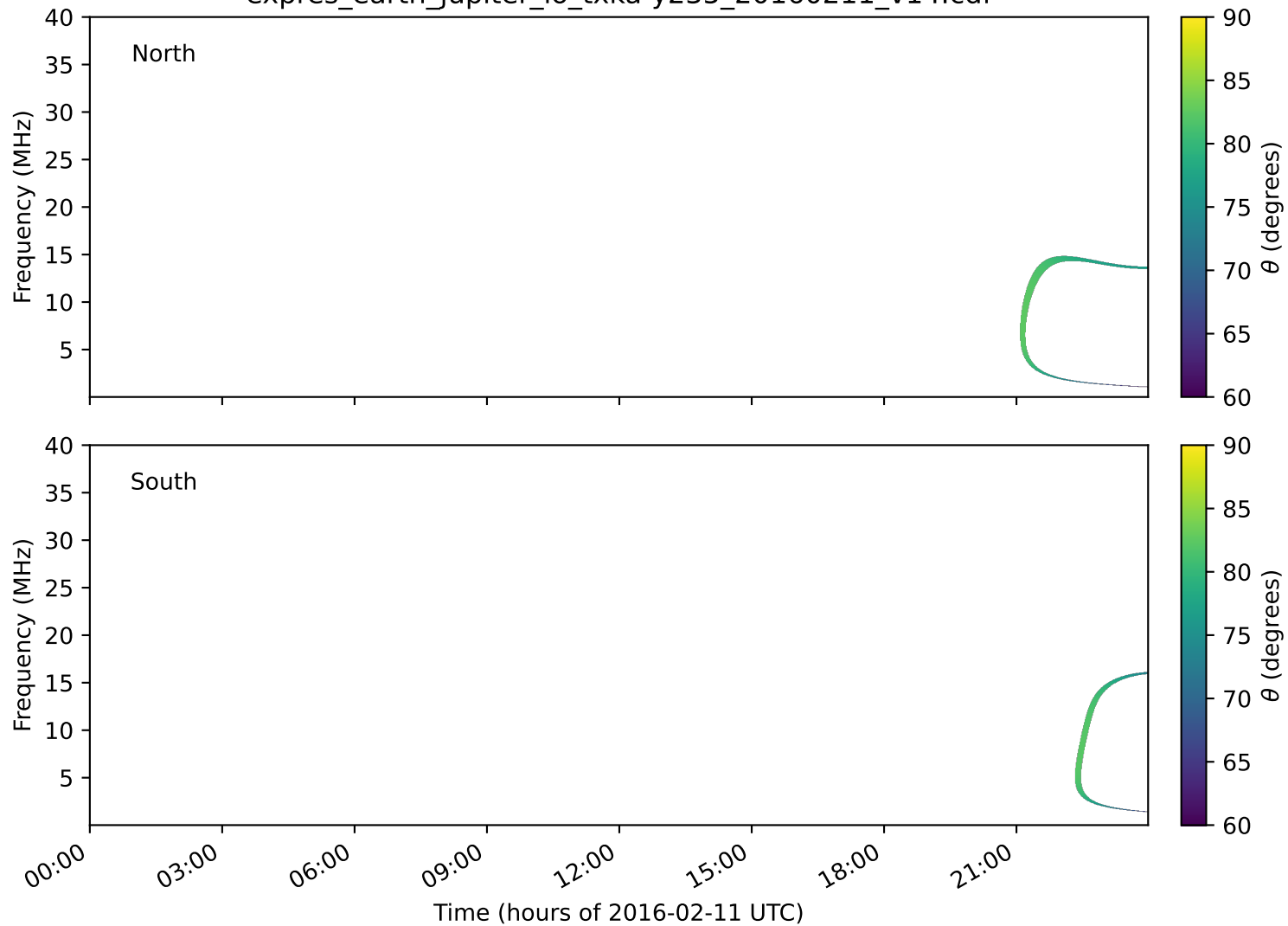
expres_earth_jupiter_io_txka-y235_20160211_v14.cdf
