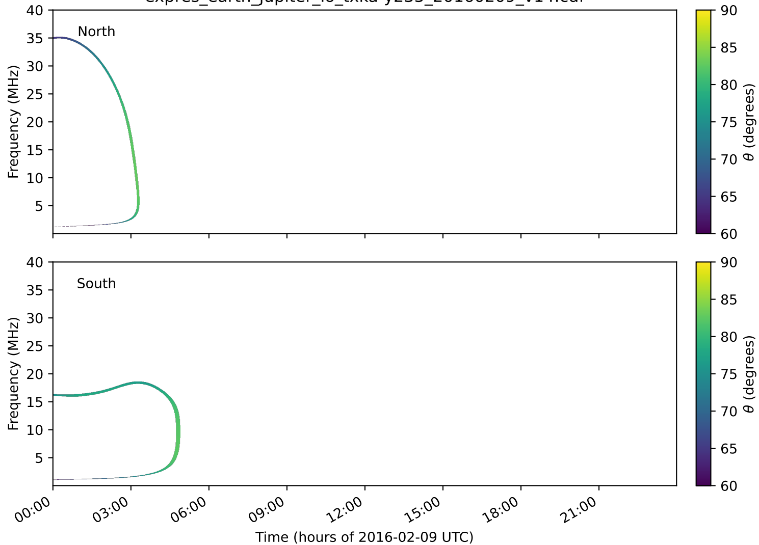
expres_earth_jupiter_io_txka-y235_20160209_v14.cdf
