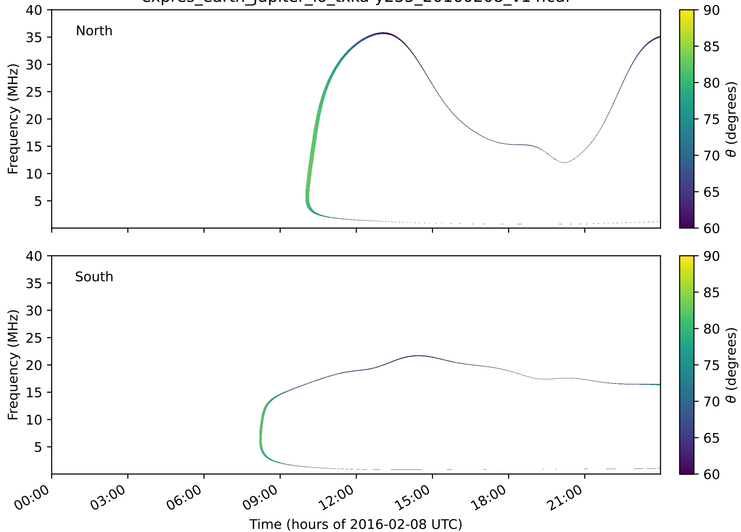
expres_earth_jupiter_io_txka-y235_20160208_v14.cdf
