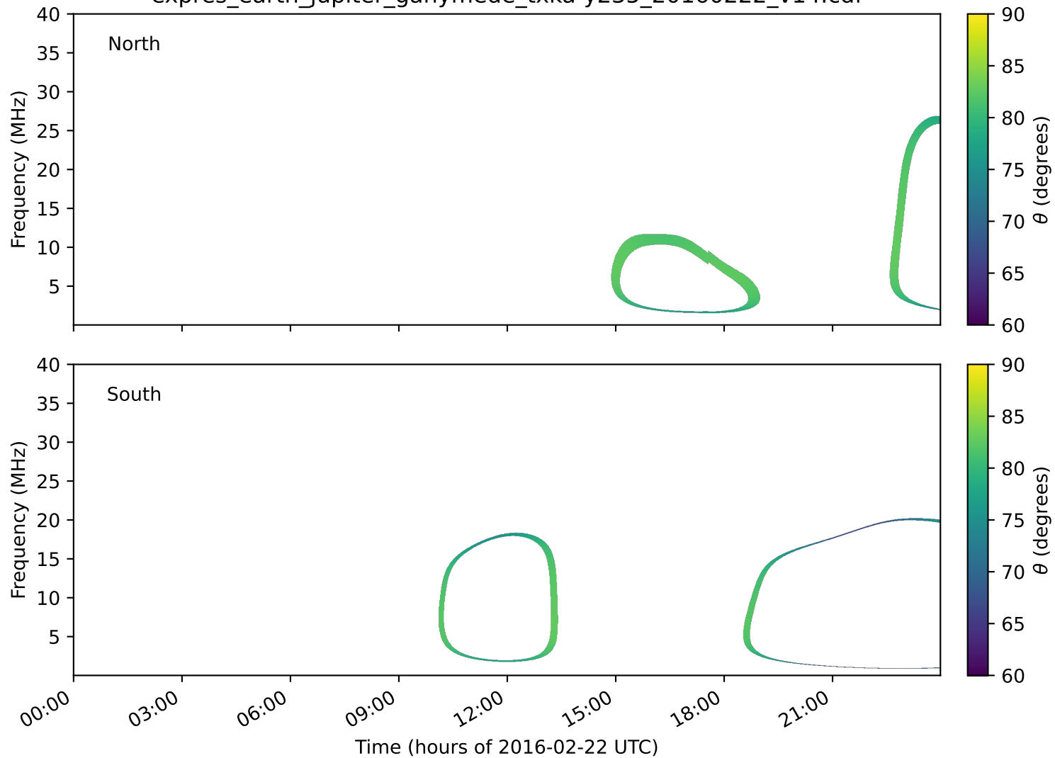
expres_earth_jupiter_ganymede_txka-y235_20160222_v14.cdf
