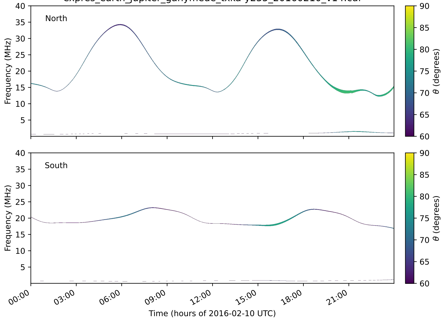
expres_earth_jupiter_ganymede_txka-y235_20160210_v14.cdf
