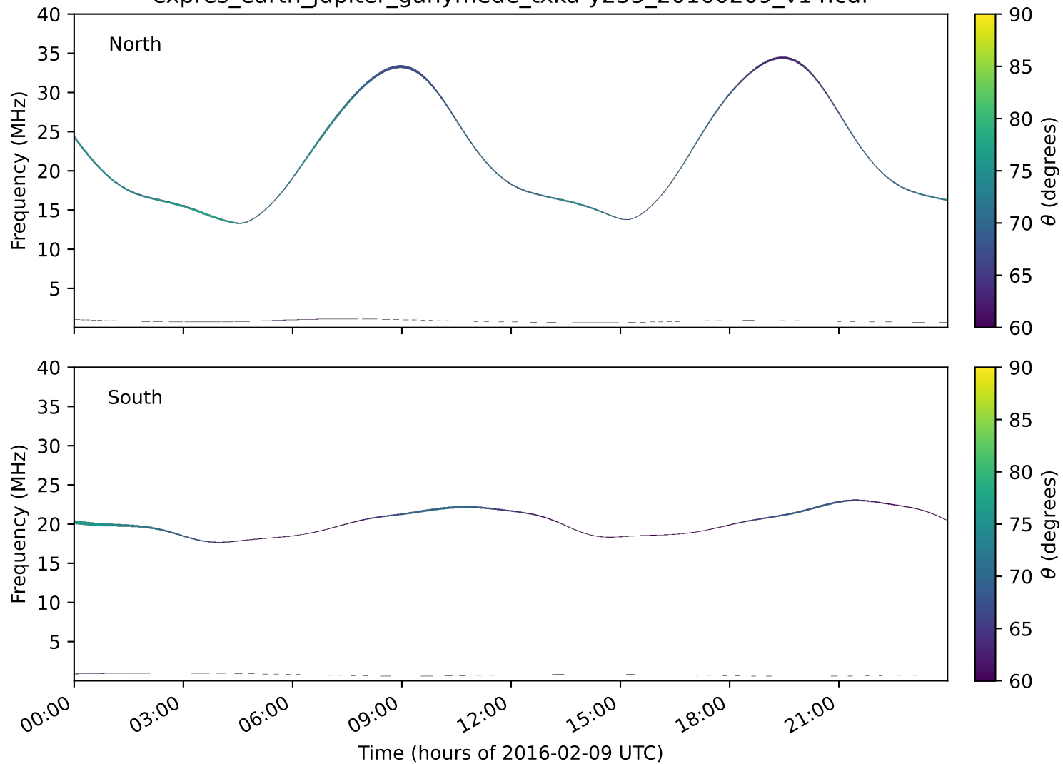
expres_earth_jupiter_ganymede_txka-y235_20160209_v14.cdf
