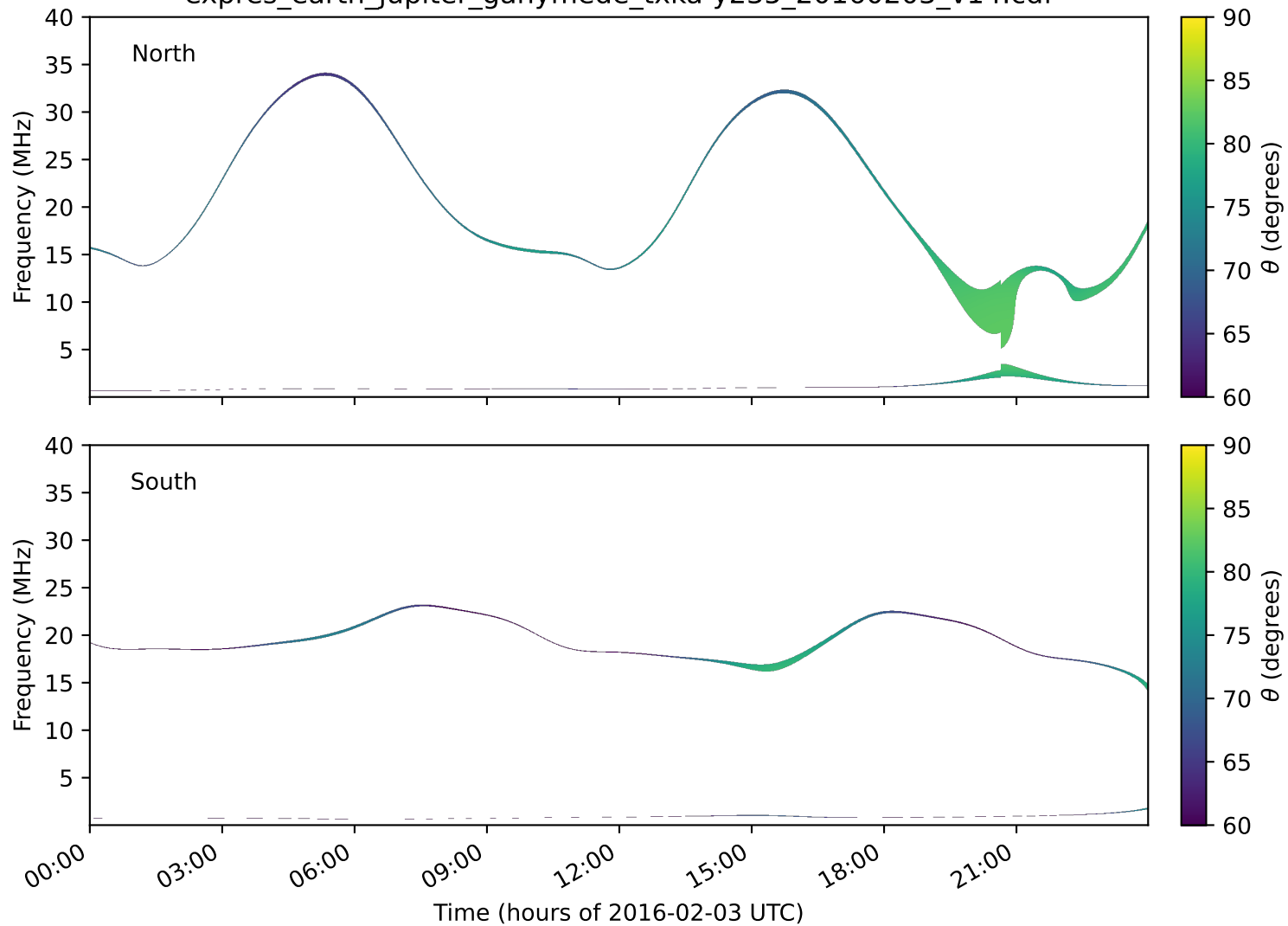
expres_earth_jupiter_ganymede_txka-y235_20160203_v14.cdf
