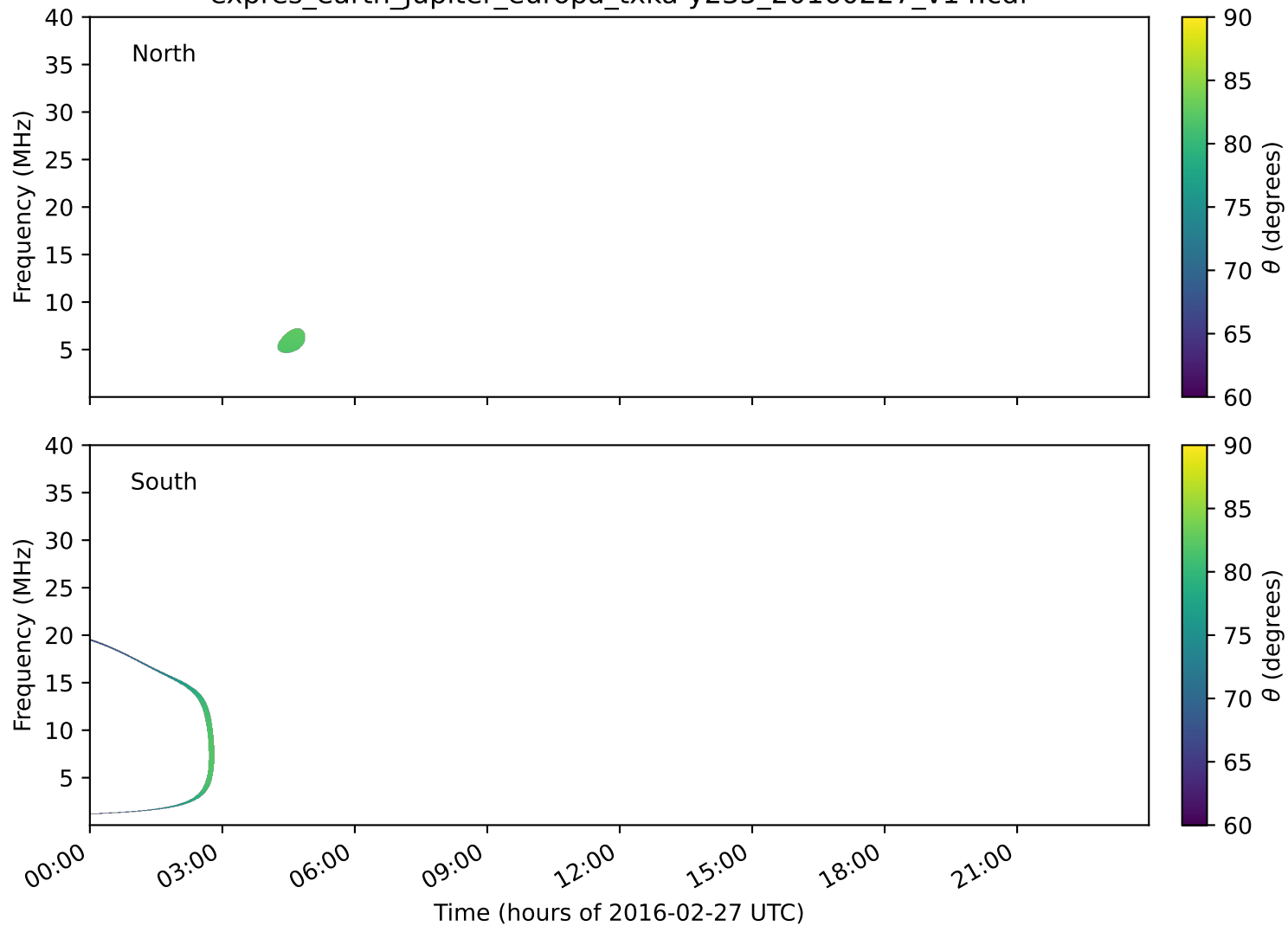
expres_earth_jupiter_europa_txka-y235_20160227_v14.cdf
