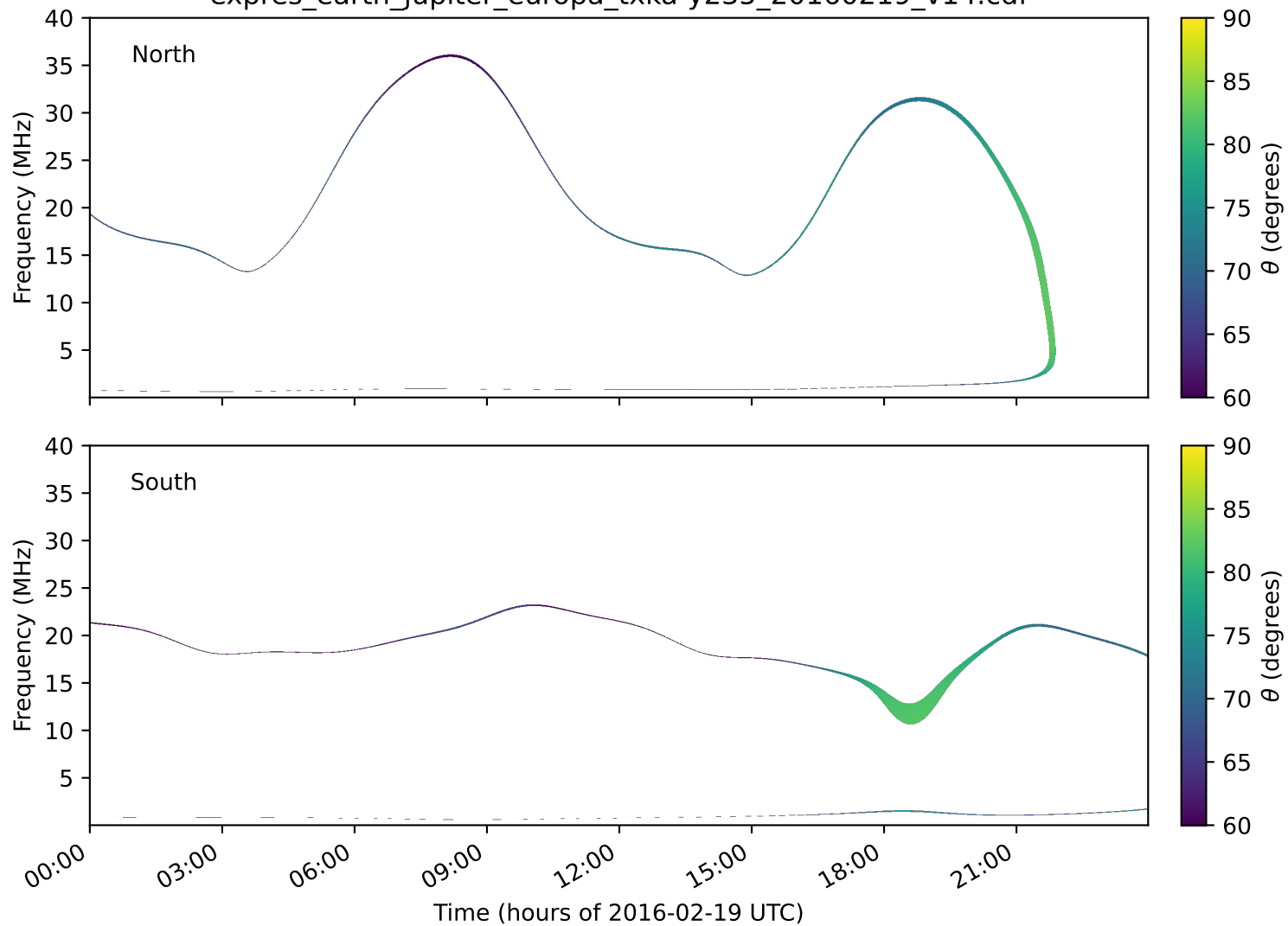
expres_earth_jupiter_europa_txka-y235_20160219_v14.cdf
