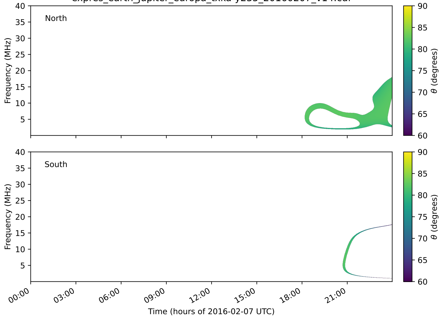
expres_earth_jupiter_europa_txka-y235_20160207_v14.cdf
