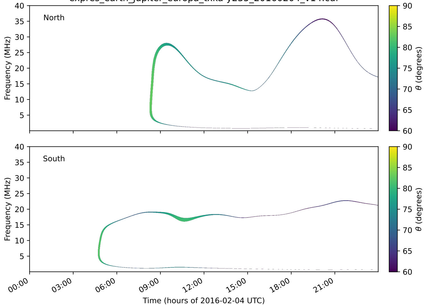
expres_earth_jupiter_europa_txka-y235_20160204_v14.cdf
