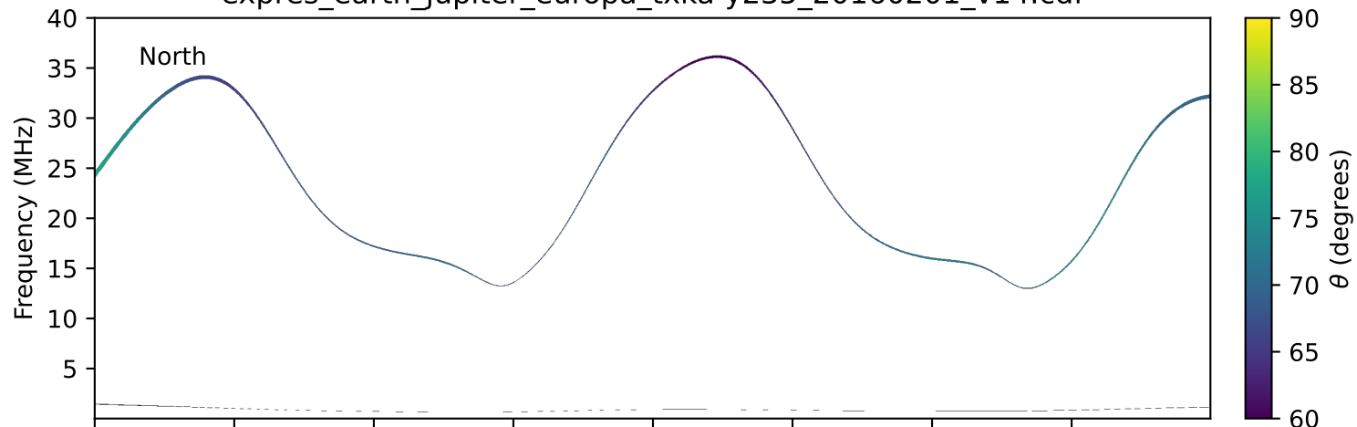
expres_earth_jupiter_europa_txka-y235_20160201_v14.cdf
