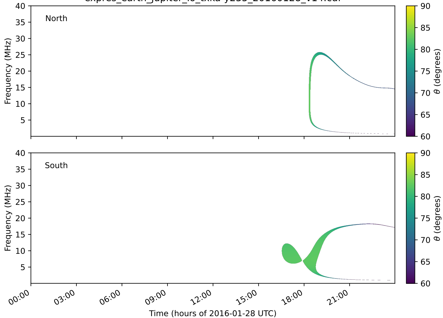
expres_earth_jupiter_io_txka-y235_20160128_v14.cdf
