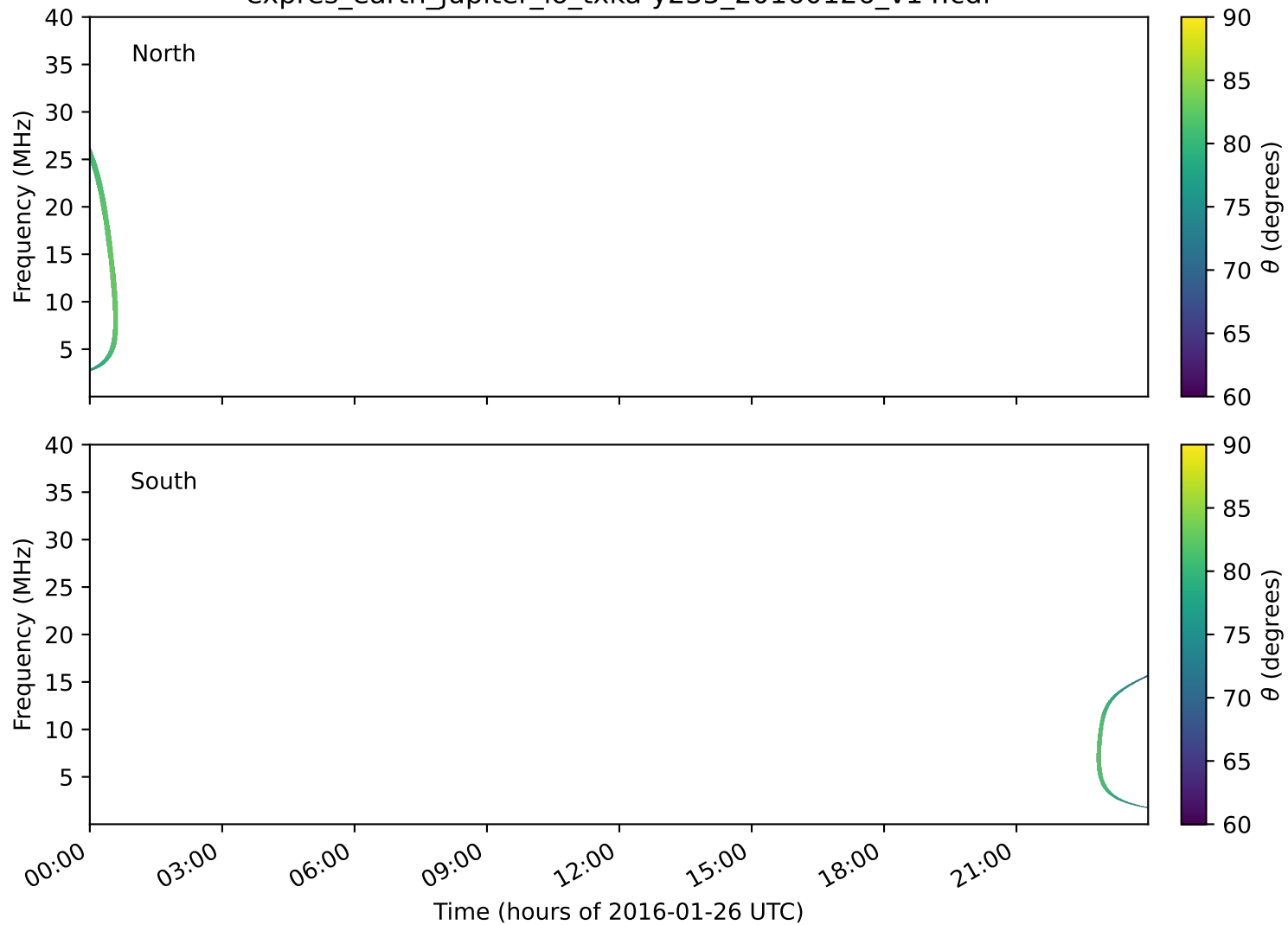
expres_earth_jupiter_io_txka-y235_20160126_v14.cdf
