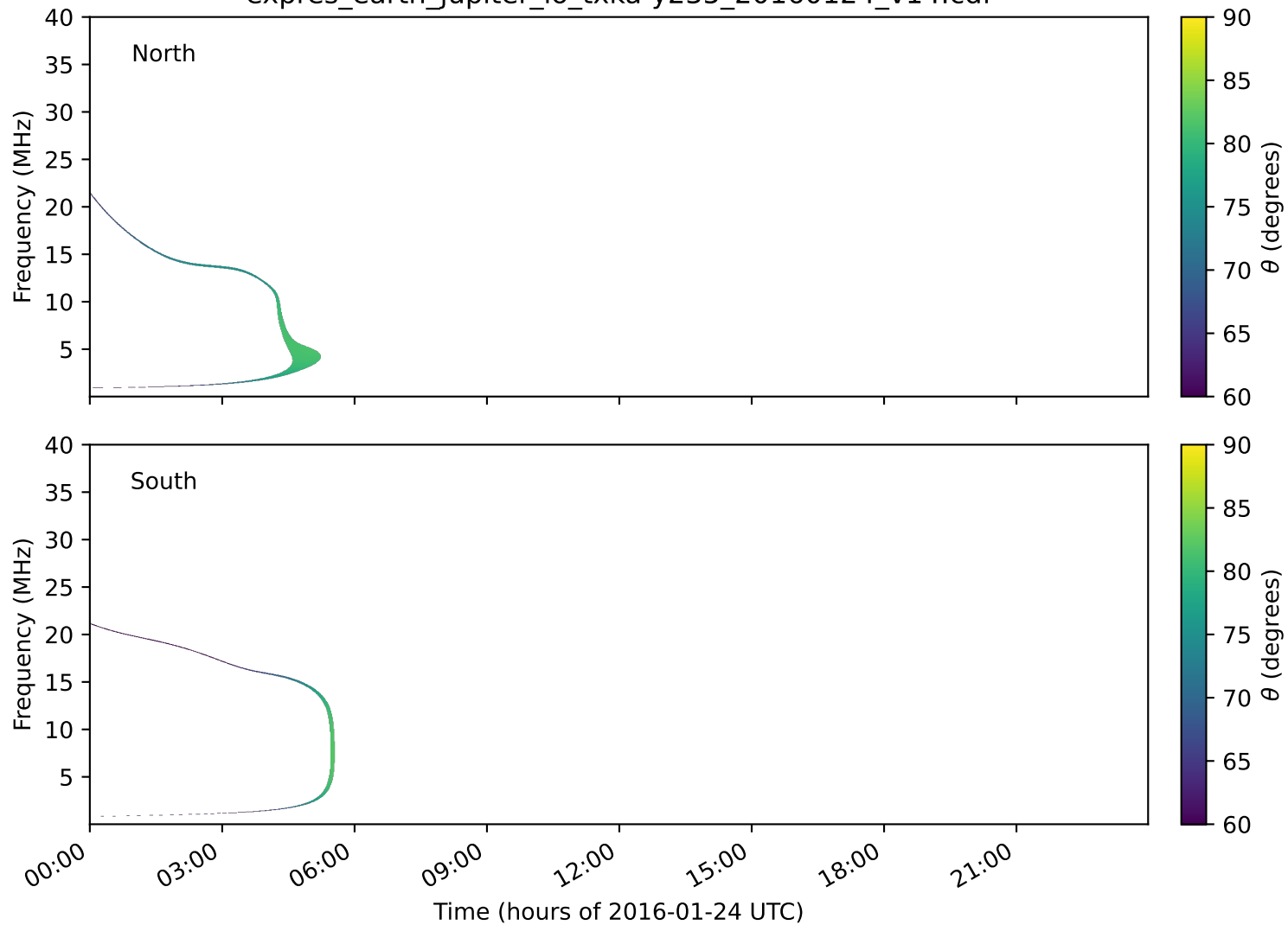
expres_earth_jupiter_io_txka-y235_20160124_v14.cdf
