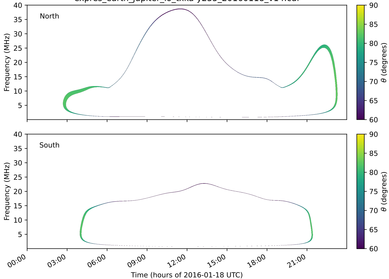
expres_earth_jupiter_io_txka-y235_20160118_v14.cdf
