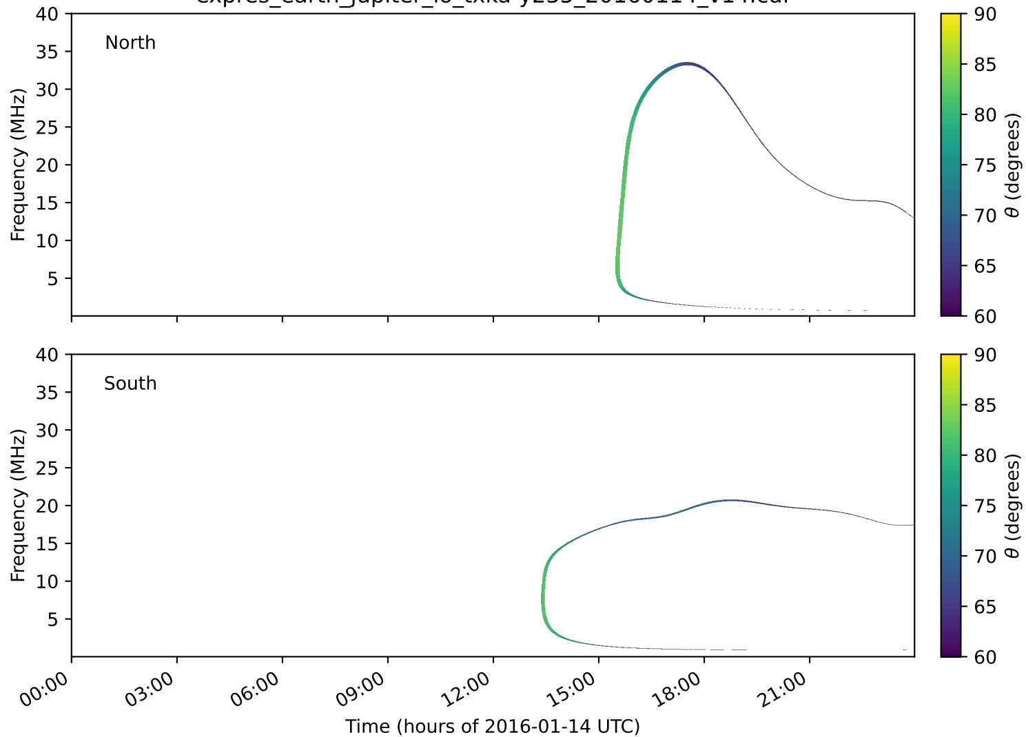
expres_earth_jupiter_io_txka-y235_20160114_v14.cdf
