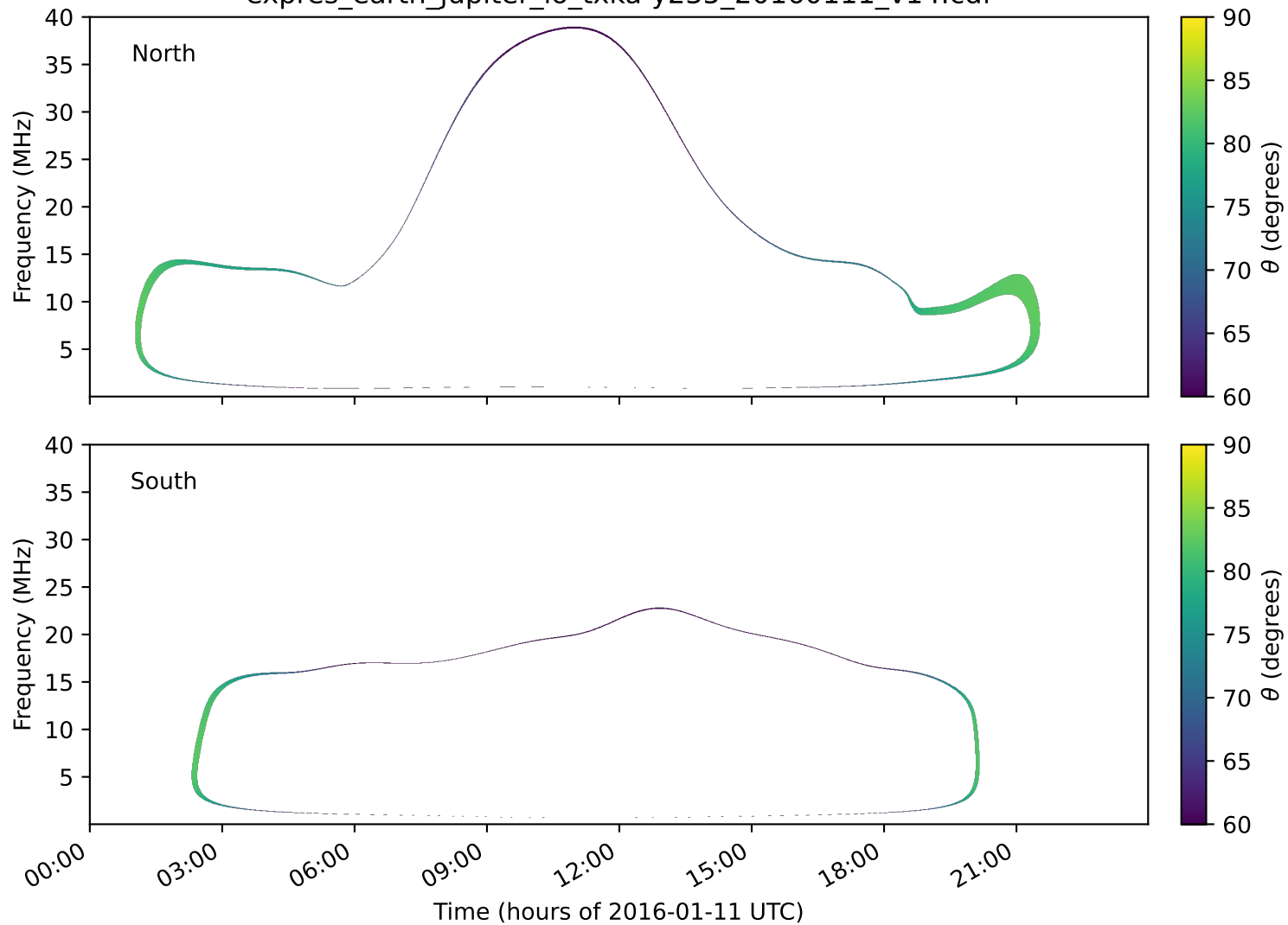
expres_earth_jupiter_io_txka-y235_20160111_v14.cdf
