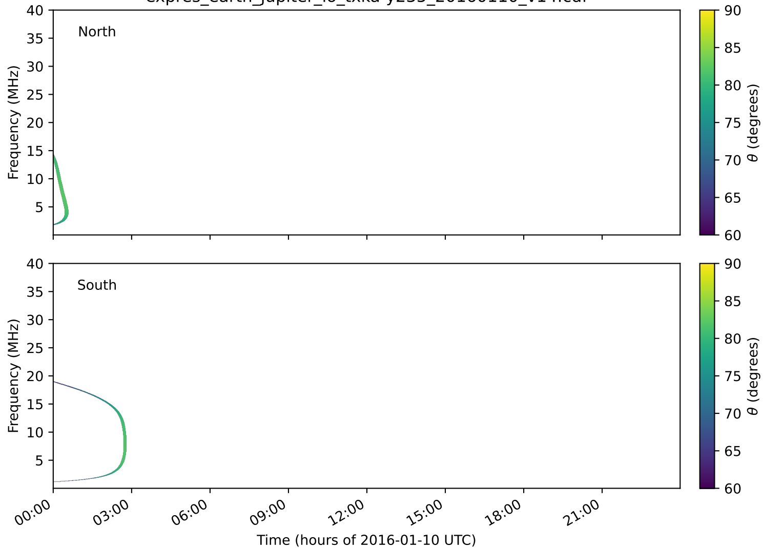
expres_earth_jupiter_io_txka-y235_20160110_v14.cdf
